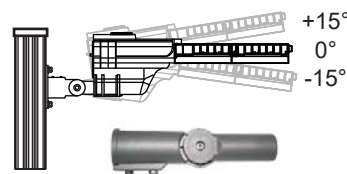
Side-Entry Position
