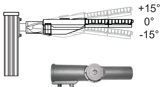
Side-Entry Position
