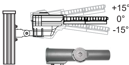
Side-Entry Position
