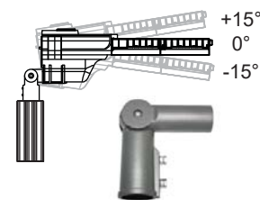
Post-Top Position
