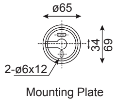
Mounting Plate
