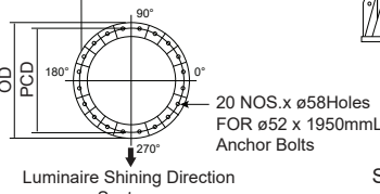
Flange Plate Stiffened with Gusset Plate
