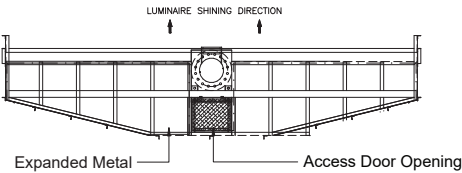
Platform Plan
