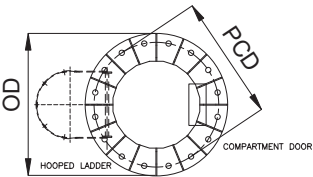
Base Flange Stiffened with Gusset
